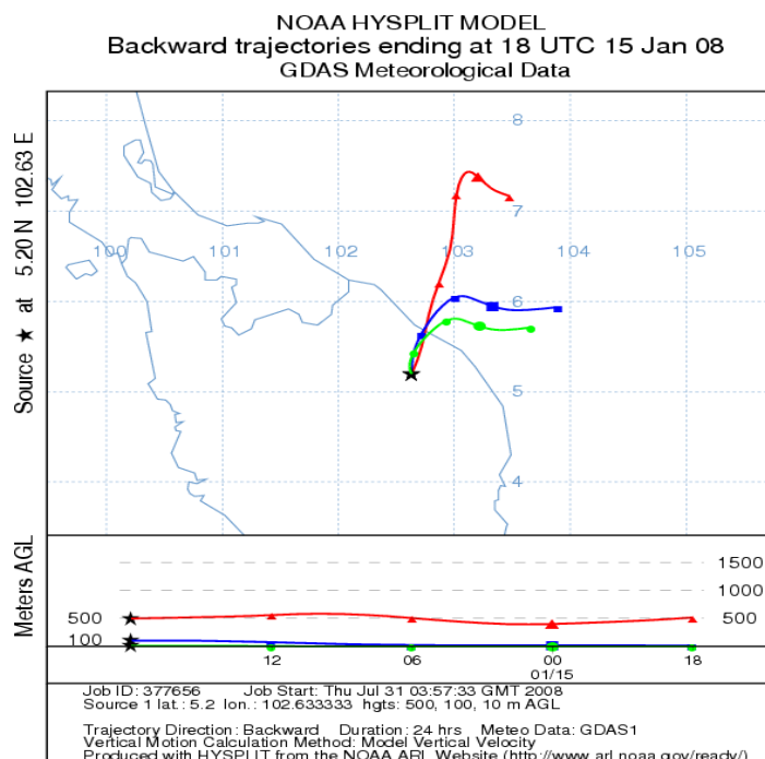
Figure 2: Backward trajectories
