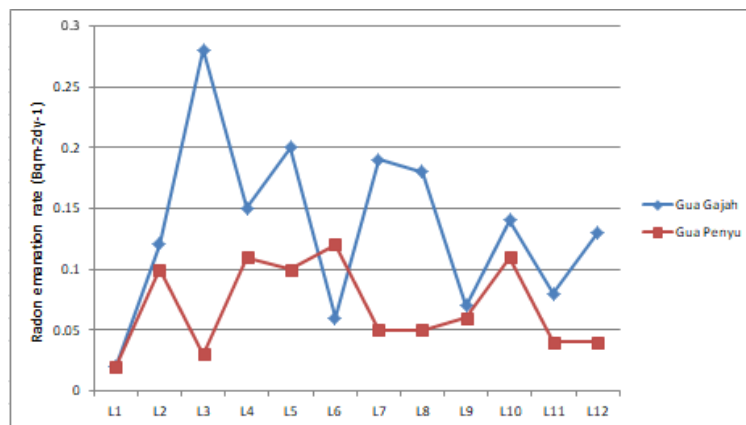
Figure 4. The Radon-222 emanation rates in Gua Gajah and Gua Penyu caves
