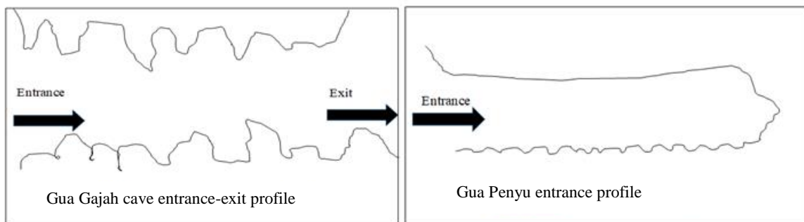
Figure 1. The sideview illustration of Gua Penyu and Gua Gajah caves entrance – exit profiles
