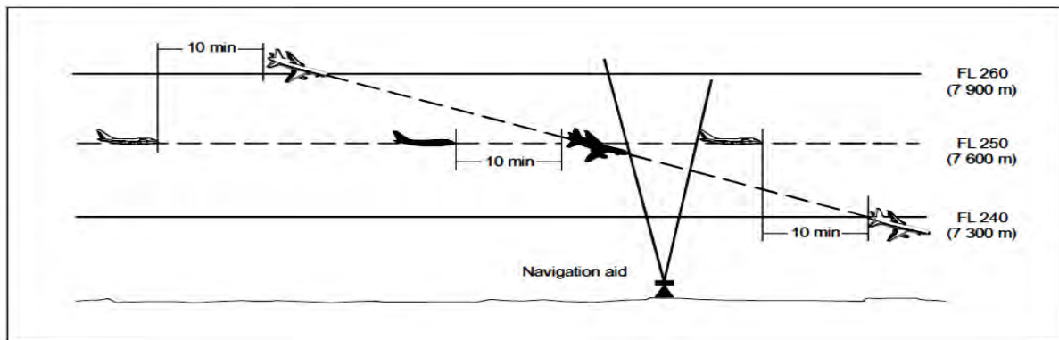
Figure 5-20B. Ten-minute separation between aircraft descending and on crossing tracks (see 5.4.2.2.2 b)
