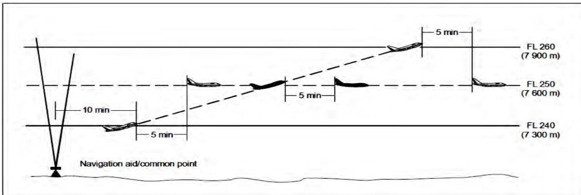
Figure 5-18A. Five-minute separation between aircraft climbing and on same track (see 5.4.2.2.1 c) 2))
