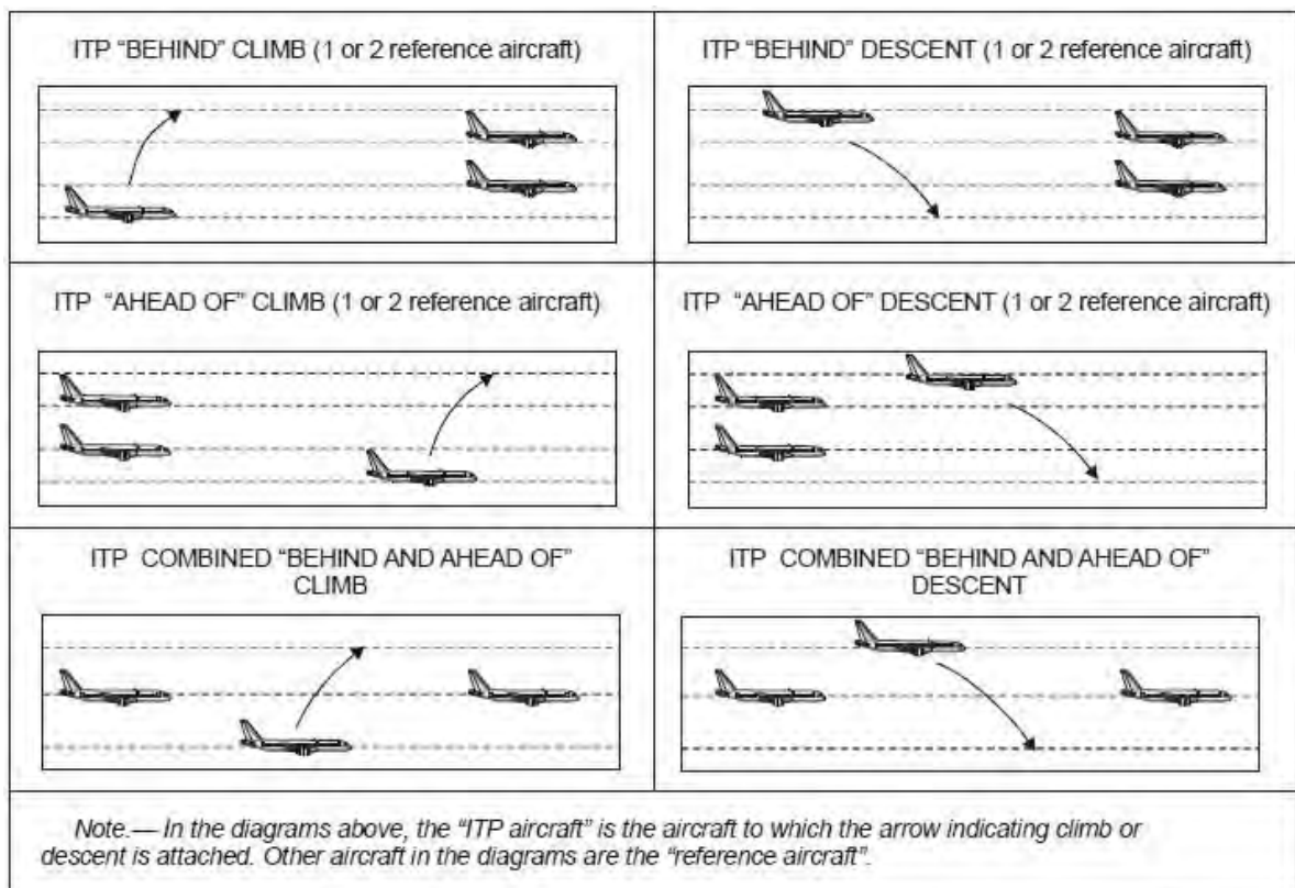
Figure 5-35. ITP flight level change scenarios (see 5.4.2.7.3)
