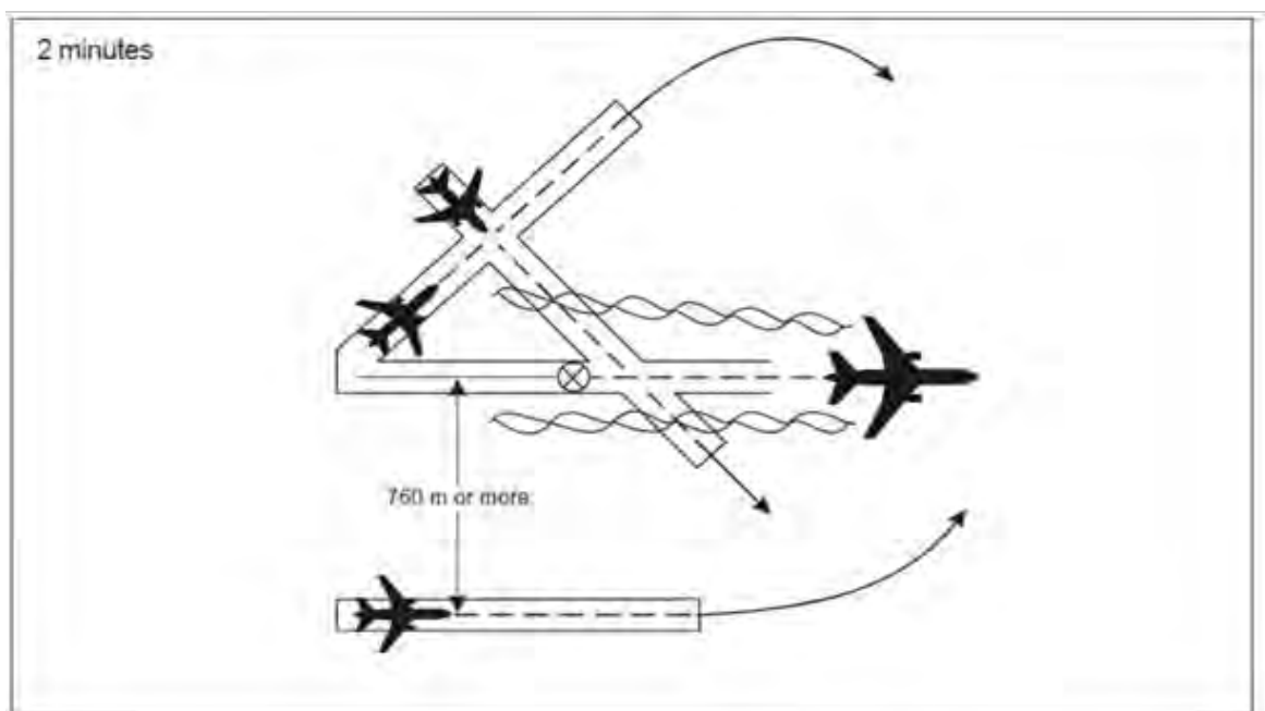
Figure 5-43. Two-minute wake turbulence separation for crossing aircraft (see 5.8.3.1c and d)
