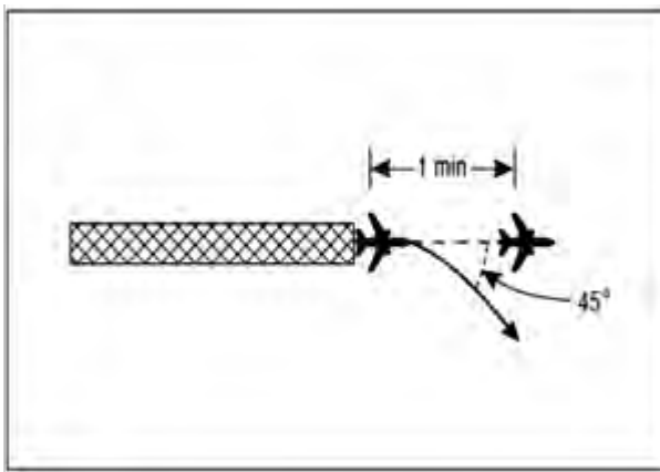
Figure 5-37. One-minute separation between departing aircraft following tracks diverging by at least 45 degrees (see 5.6.1)
