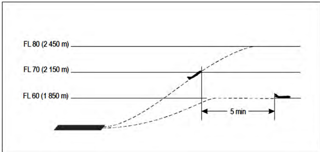
Figure 5-39. Five-minute separation of departing aircraft following the same track (see 5.6.3)
