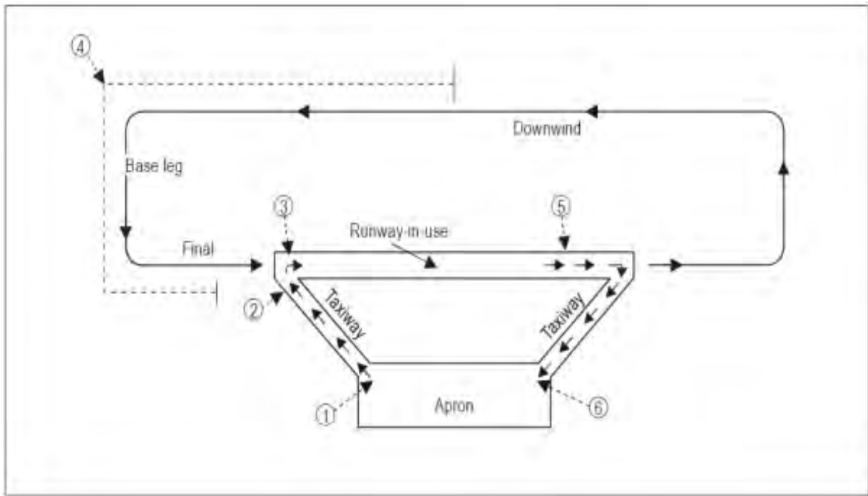
Figure 7-1. Designated positions of aircraft from an aerodrome control tower viewpoint (see 7.6.2)
