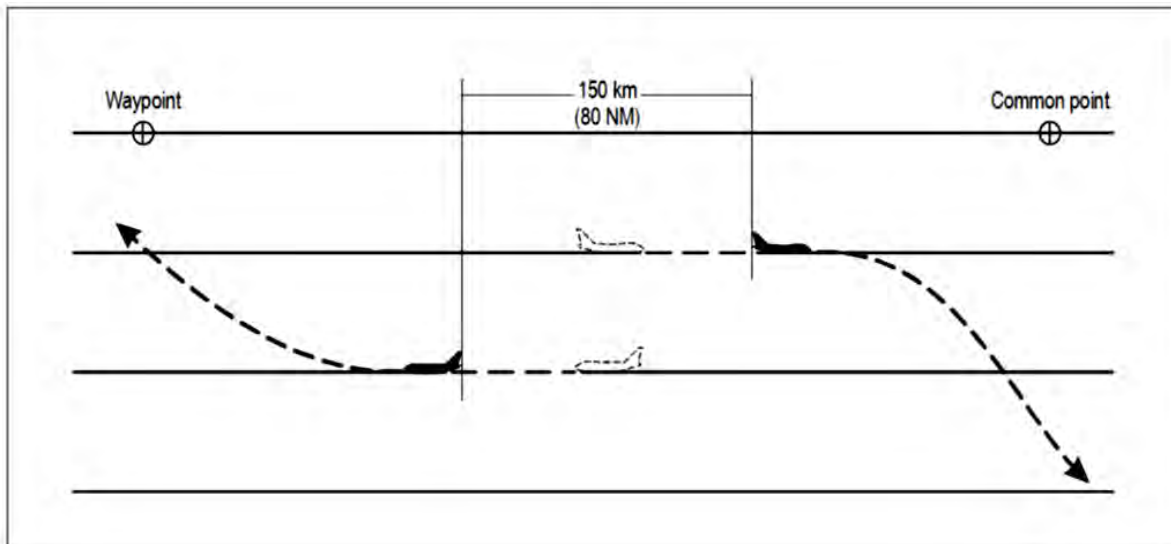
Figure 5-28. 150 km (80 NM) RNAV-based separation between aircraft on reciprocal tracks (see 5.4.2.5.7))
