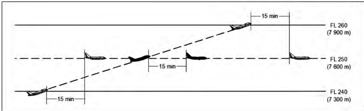
Figure 5-16A. Fifteen-minute separation between aircraft climbing and on same track (see 5.4.2.2.2.1 a)
