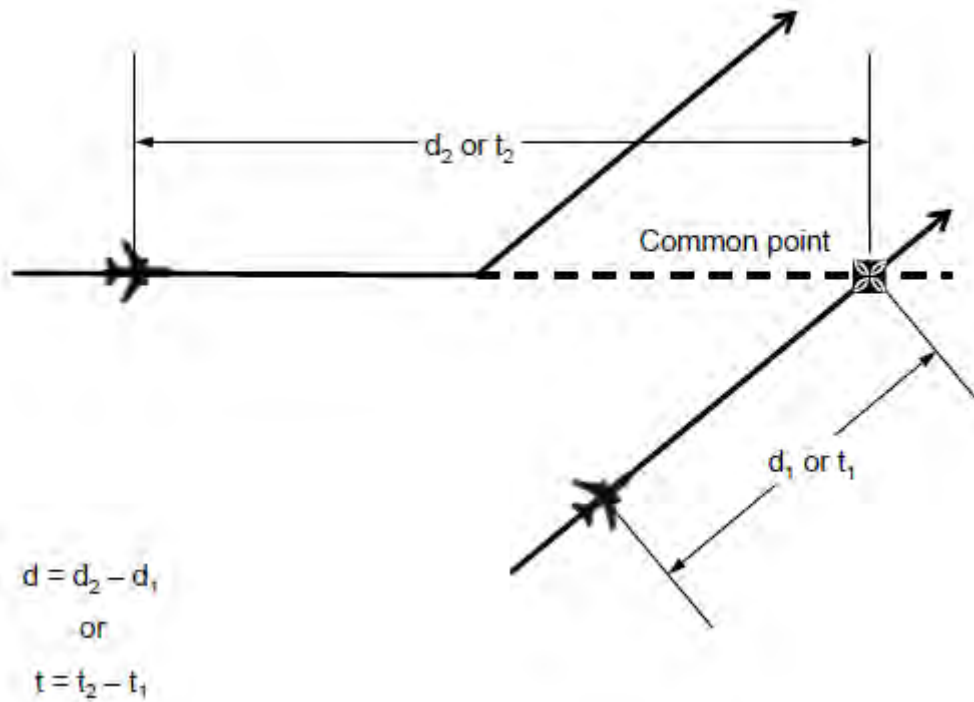
Figure 5-32. Calculation of longitudinal distance/time between aircraft — same track projected, but not identical (see 5.4.2.9.5 b)
