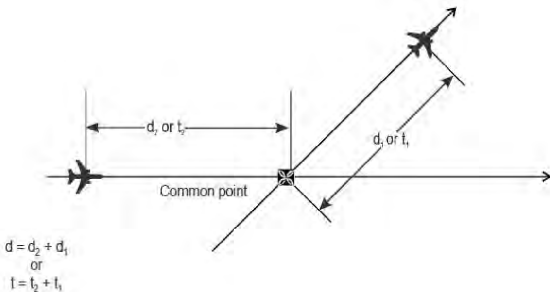
Figure 5-33. Calculation of longitudinal distance/time between aircraft — opposite sides of the common point (see 5.4.2.9.5 b)
