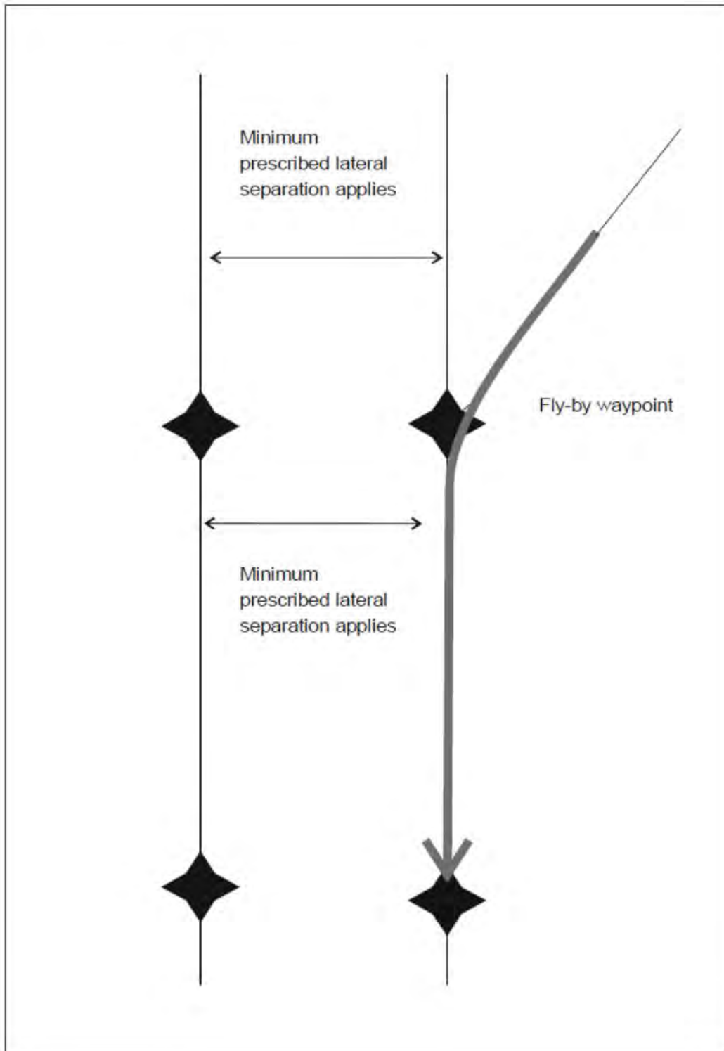
Figure 5-2. Turn at fly-by waypoint (see 5.4.1.1.4)
