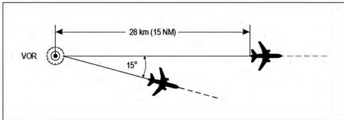
Figure 5-4. Separation using the same VOR (see 5.4.1.2.1.2 a)
