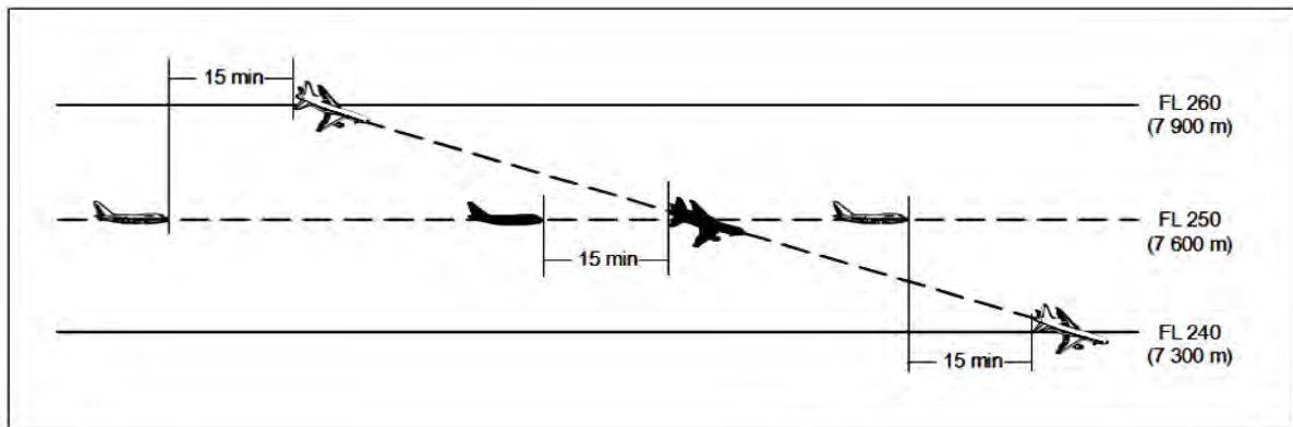
Figure 5-19B. Fifteen-minute separation between aircraft descending and on crossing tracks (see 5.4.2.2.2.2 a))
