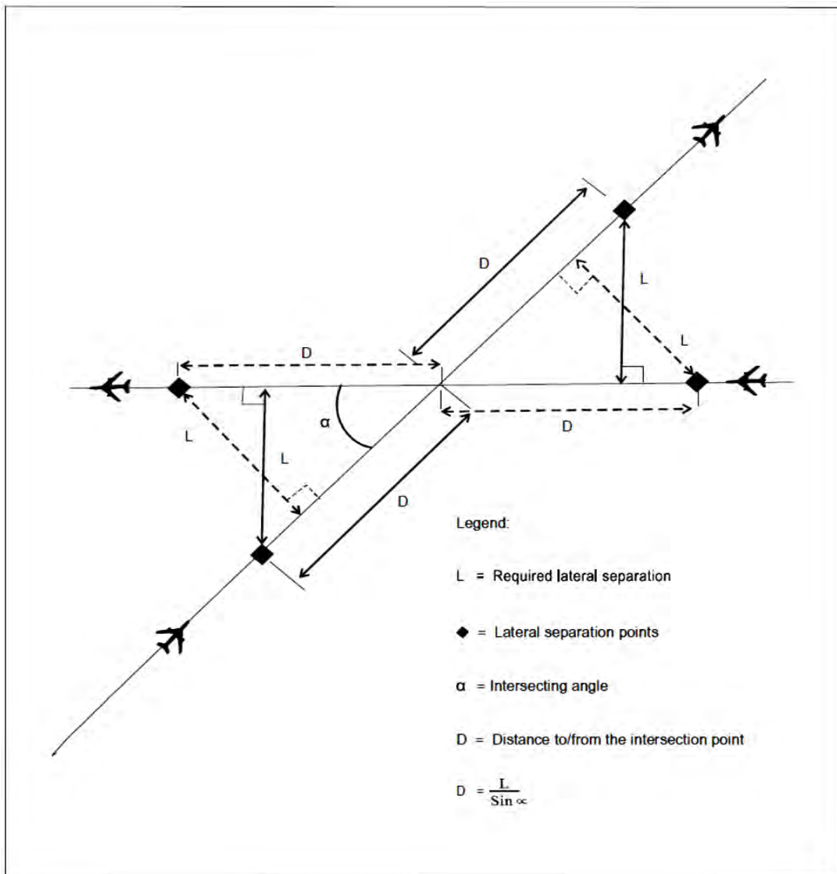
Figure 5-6. Lateral separation points (see 5.4.1.2.1.7)
