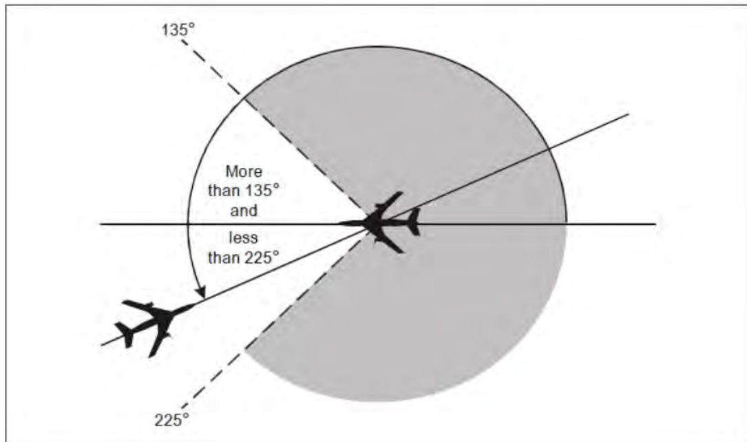
Figure 5-9. Aircraft on crossing tracks (see 5.4.2.1.5 c)
