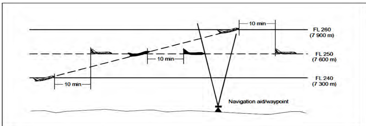
Figure 5-17A. Ten-minute separation between aircraft climbing and on same track (see 5.4.2.2.2.1 b)
