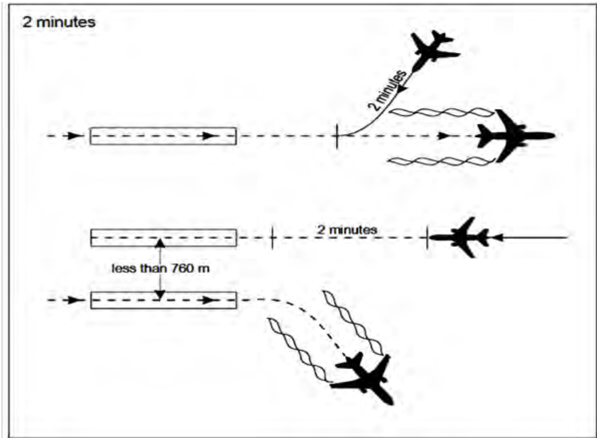
Figure 5-45. Two-minute wake turbulence separation for opposite direction take-off (see 5.8.5 a)
