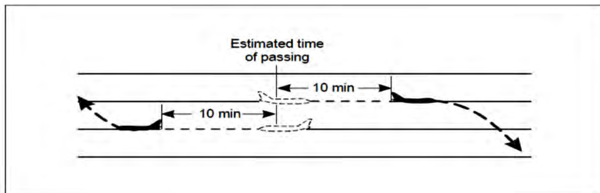
Figure 5-21. Ten-minute separation between aircraft on reciprocal tracks (see 11.4.2.2.3)
