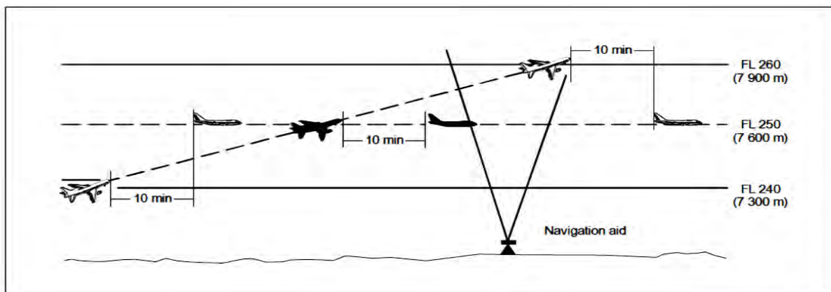
Figure 5-20A. Ten-minute separation between aircraft climbing and on crossing tracks (see 5.4.2.2.2.2 b))
