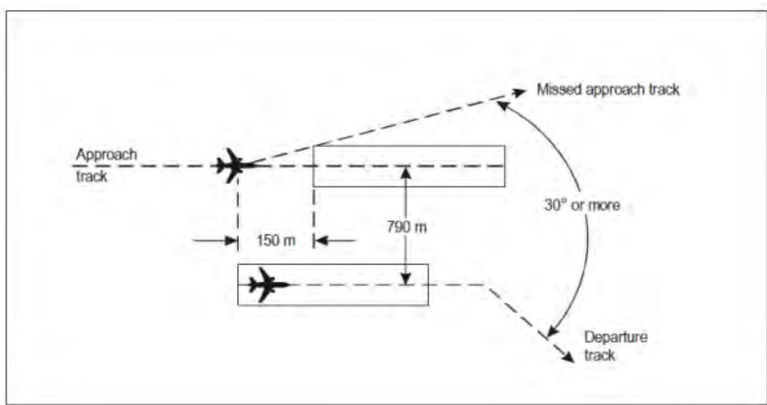
Figure 6-3. Segregated Parallel Operations where runways are staggered (see 6.7.3.5.2)
