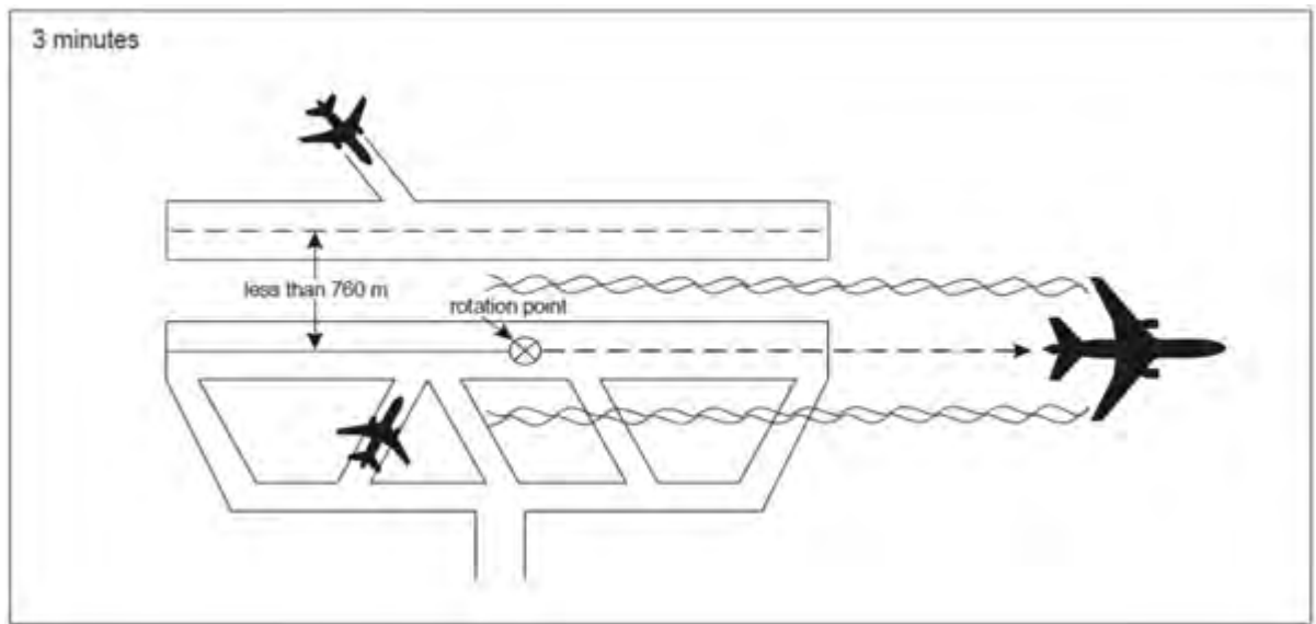
Figure 5-44. Three-minute wake turbulence separation for following aircraft (see 5.8.3.2)
