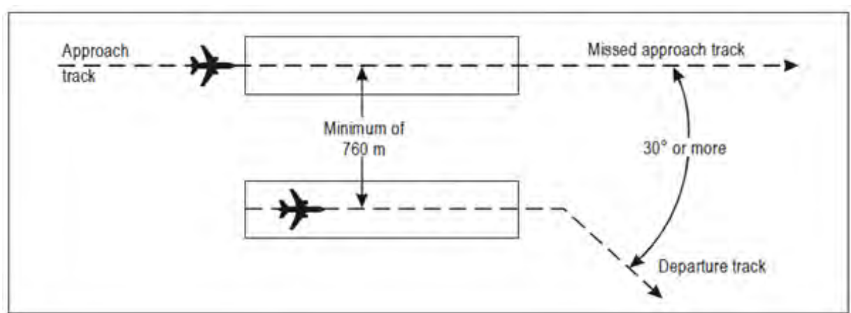
Figure 6-1. Segregated Parallel Operations (see 6.7.3.5.1 b)
