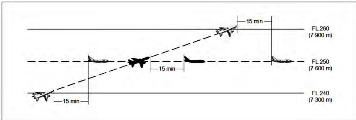
Figure 5-19A. Fifteen-minute separation between aircraft climbing and on crossing tracks (see 5.4.2.2.2.2 a))
