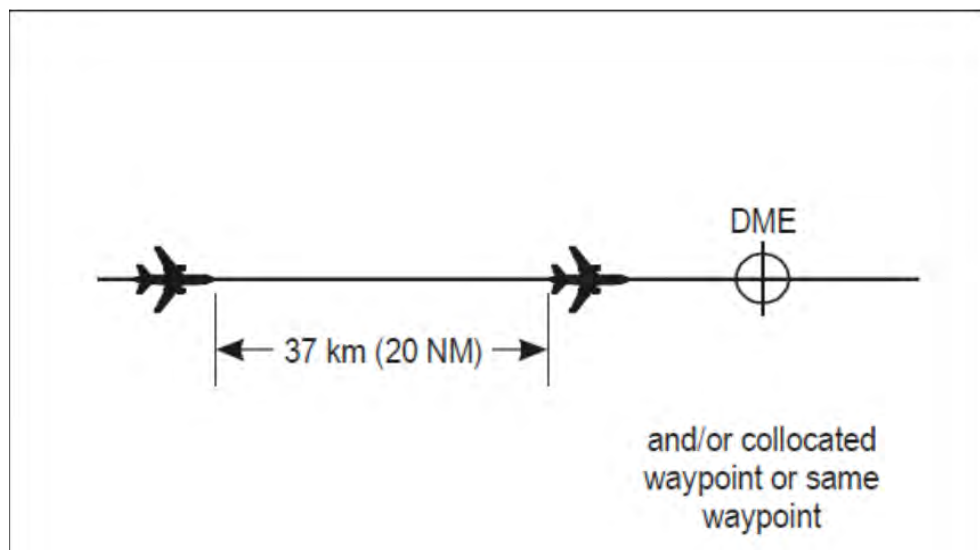
Figure 5-22. 37 km (20 NM) DME and/or GNSS-based separation between aircraft on same track and same level (see 5.4.2.3.3.1 a))
