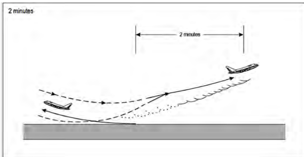
Figure 5-46. Two-minute wake turbulence separation for opposite direction landing (see 5.8.5 b)
