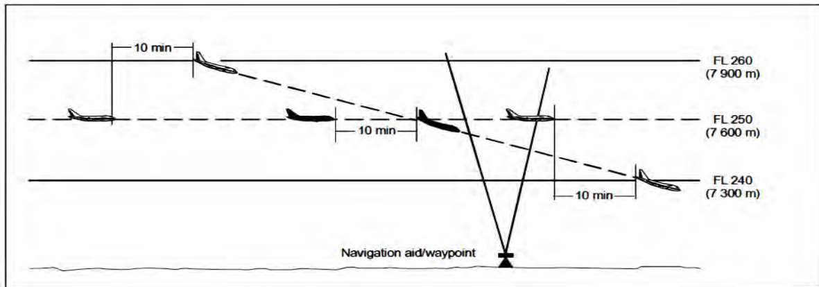
Figure 5-17B. Ten-minute separation between aircraft descending and on same track (see 5.4.2.2.1 b)
