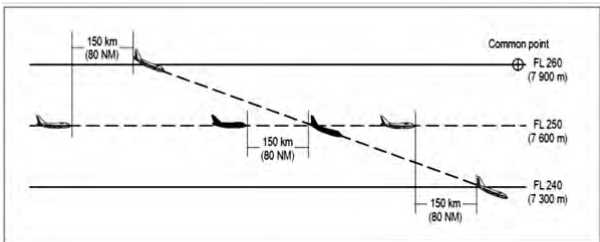
Figure 5-27B. 150 km (80 NM) RNAV-based separation between aircraft descending and on same track (see 5.4.2.5.5 c)
