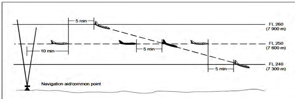
Figure 5-18B. Five-minute separation between aircraft descending and on same track (see 5.4.2.2.1 c) 2))
