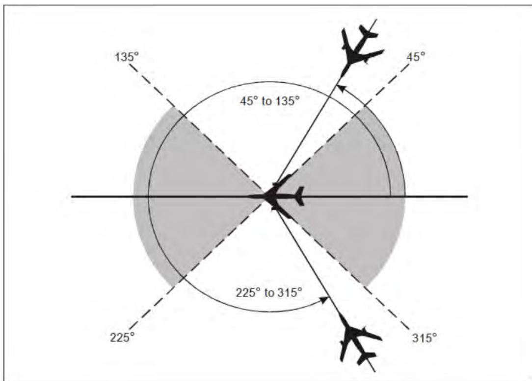
Figure 5-8. Aircraft on reciprocal tracks (see 5.4.2.1.5.b)
