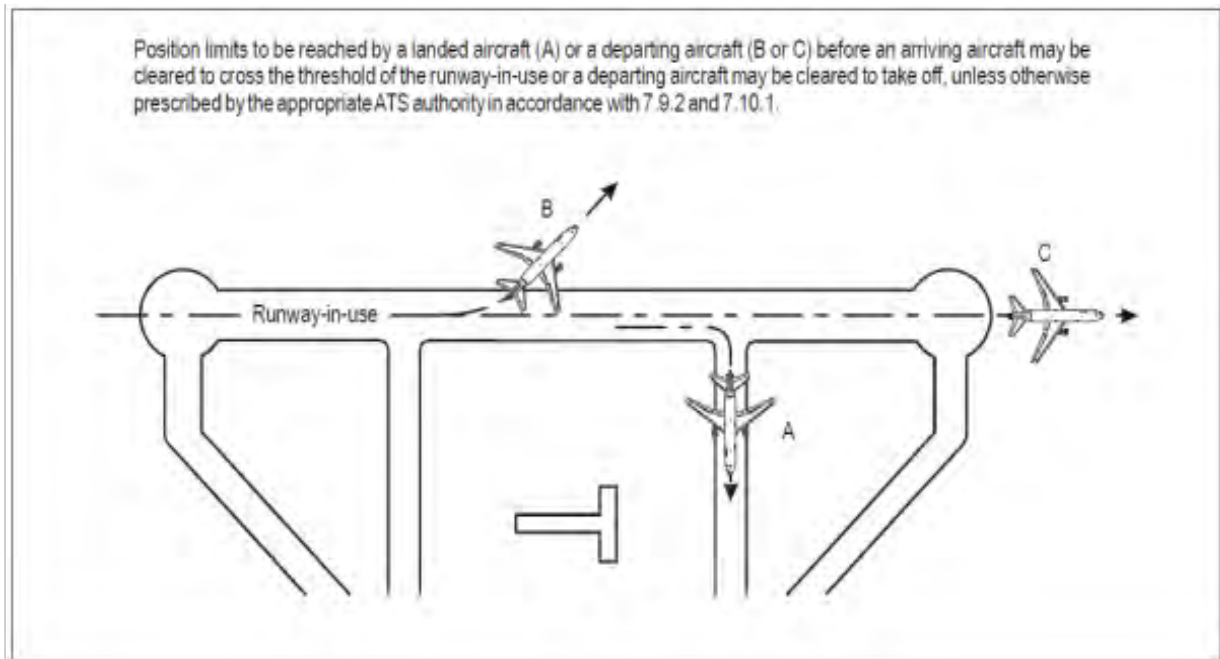
Figure 7-3. Separation between departing and arriving aircraft (see 7.9.2 and 7.10.1)
