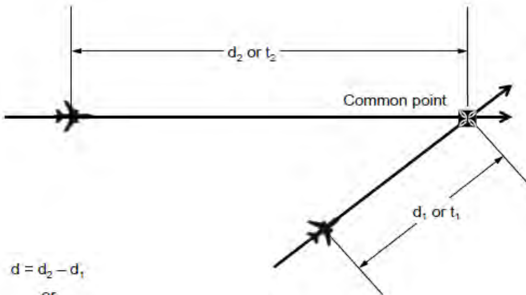
Figure 5-31. Calculation of longitudinal distance/time between aircraft — same track, but not identical and crossing tracks (see 5.4.2.9.5 b))
