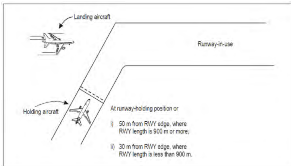
Figure 7-2. Method of holding aircraft (see 7.6.3.1.3.2)
