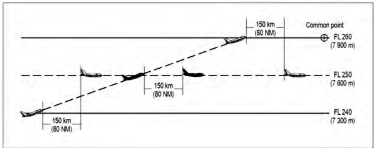
Figure 5-27A. 150 km (80 NM) RNAV-based separation between aircraft climbing and on same track (see 5.4.2.5.5 c)
