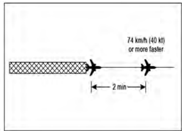
Figure 5-38. Two-minute separation between aircraft following same tracks (see 5.6.2)
