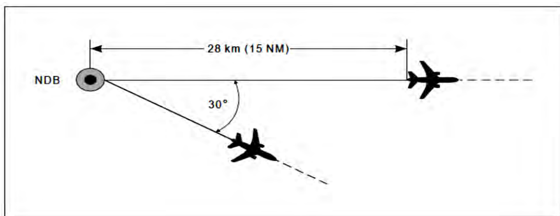
Figure 5-5. Separation using the same NDB (see 5.4.1.2.1.2.b)
