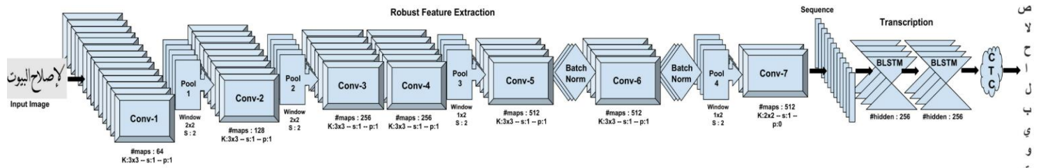
FIGURE 4. Visualization of the hybrid CNN-RNN architecture with a 7-layer-deep convolutional block (Jain 2018)
