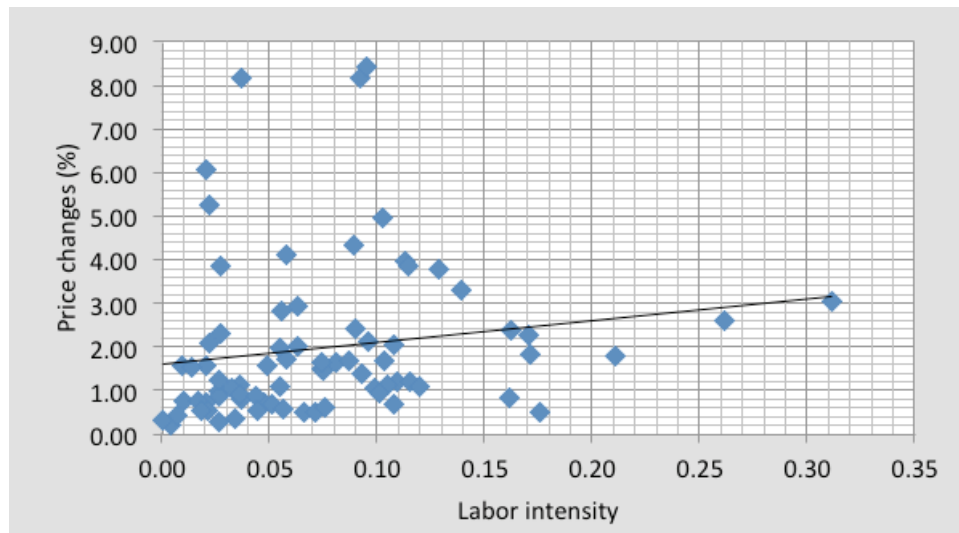
FIGURE 2. Relationship between Changes in Price and Labor Intensity Sources: Computed from the model
