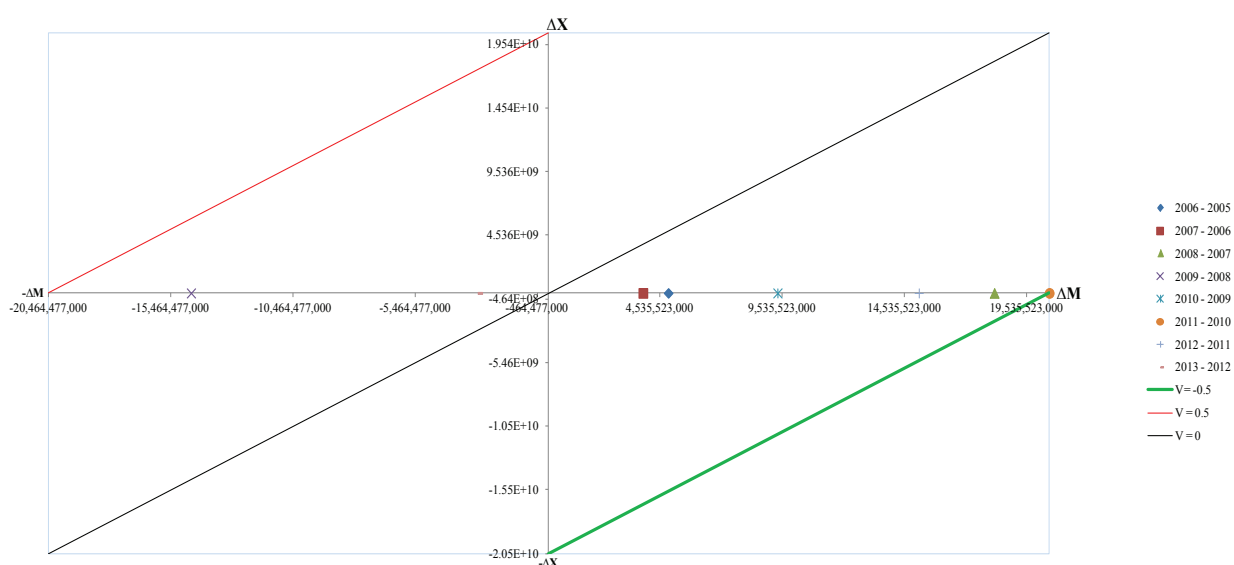
FIGURE 9. The V index diagram of Japan HS271111 first angle approach actual N data
