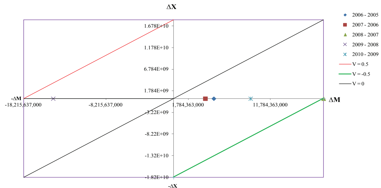
FIGURE 3. The V Index Diagram of Japan HS271111
