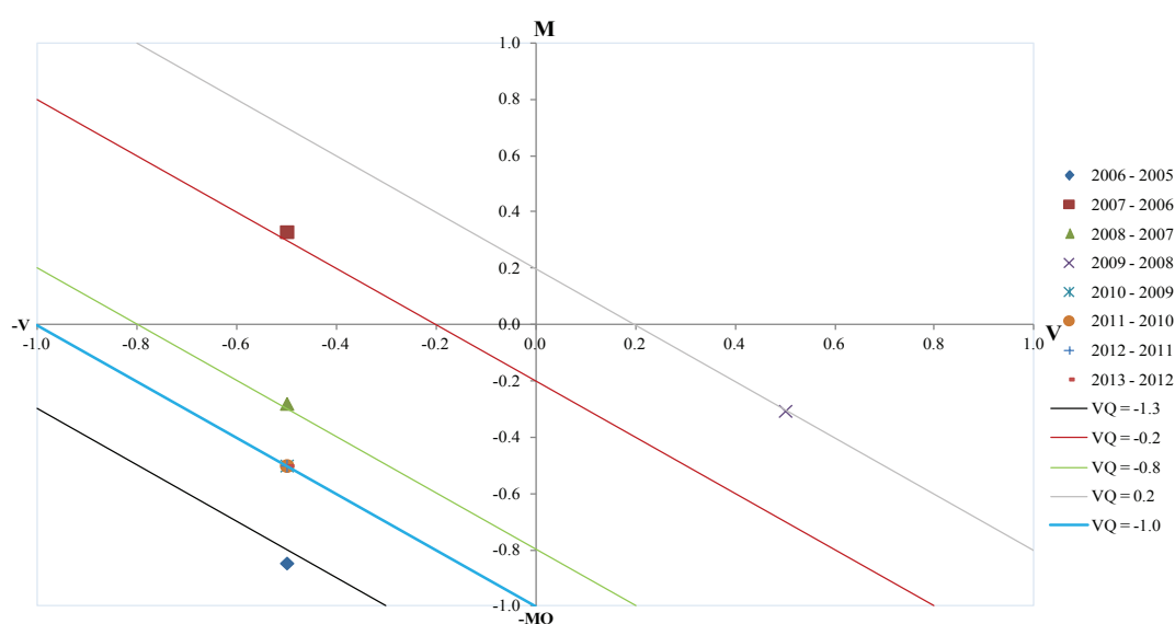
FIGURE 8. The VQ index diagram of Japan HS271111 first angle approach average calculated N data
