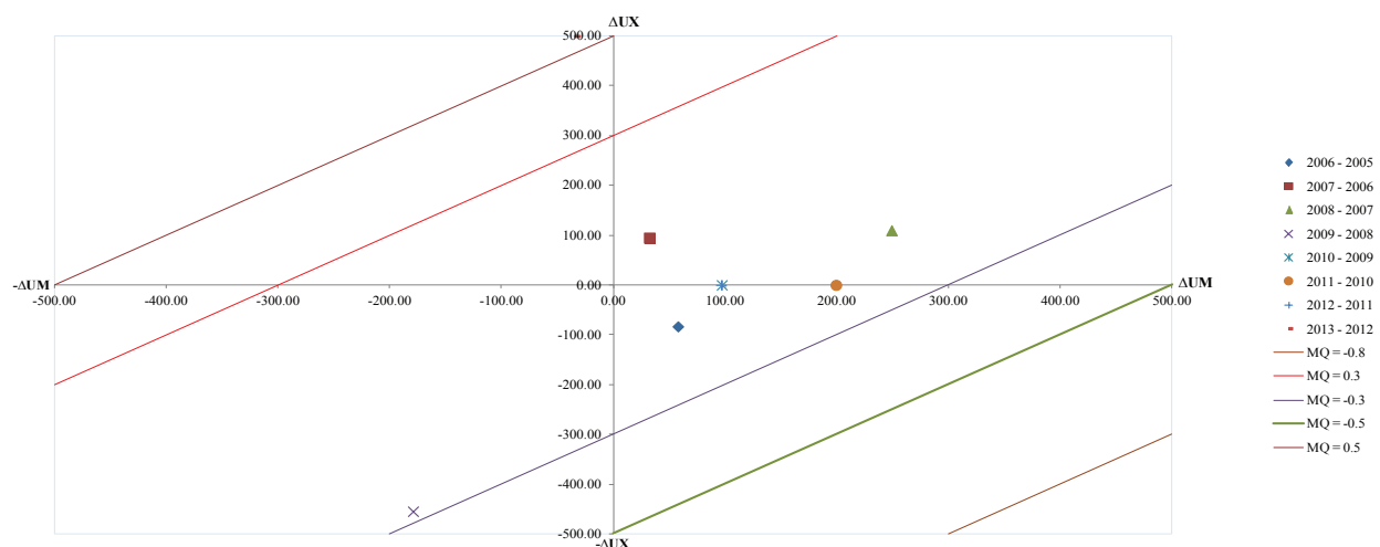
FIGURE 10. The MQ index diagram of Japan HS271111 first angle approach actual N data
