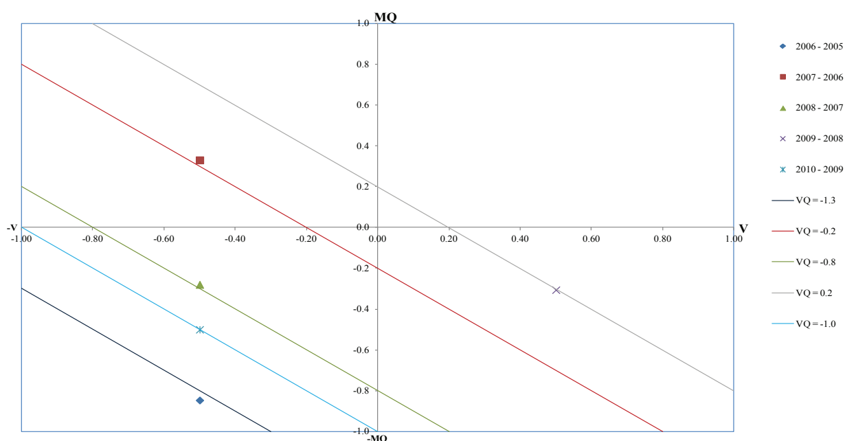
FIGURE 5. The VQ Index diagram of Japan HS271111
