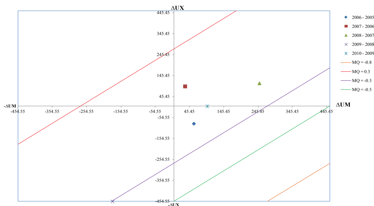
FIGURE 4. The MQ Index Diagram of Japan HS271111
