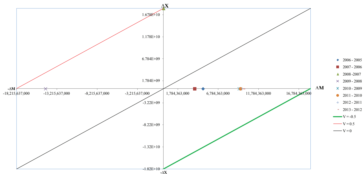
FIGURE 6. The V index diagram of Japan HS271111 first angle approach average calculated N data
