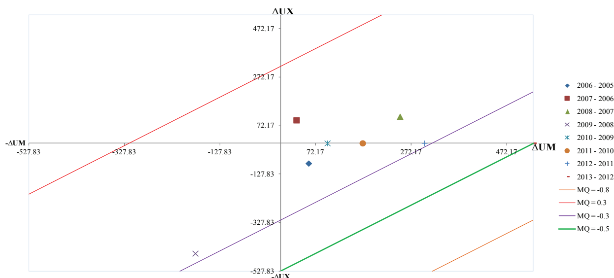
FIGURE 7. The MQ index diagram of Japan HS271111 first angle approach average calculated N data
