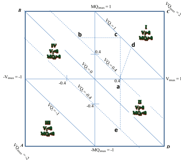
FIGURE 2. Illustration of adjusted V and MQ in GVQISB diagram Source: Azhar & Elliot (2011)
