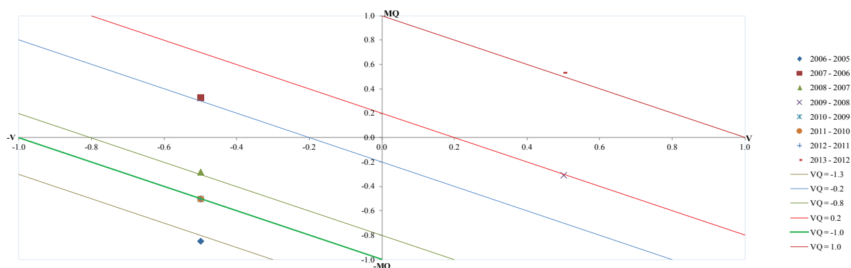
FIGURE 11. The VQ index diagram of Japan HS271111 first angle approach actual N data
