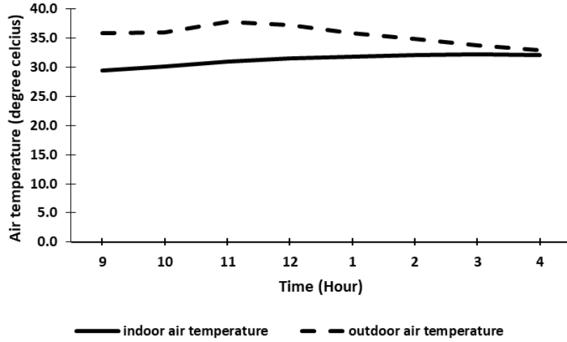
FIGURE 7. The average outdoor and indoor air temperatures
