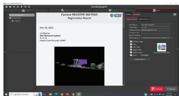
FIGURE 14. Registration report
