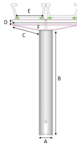
FIGURE 3. Pier elements
