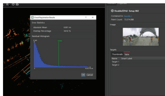
FIGURE 12. Cloud registration results
