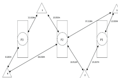
FIGURE 4. TLS setup locations
