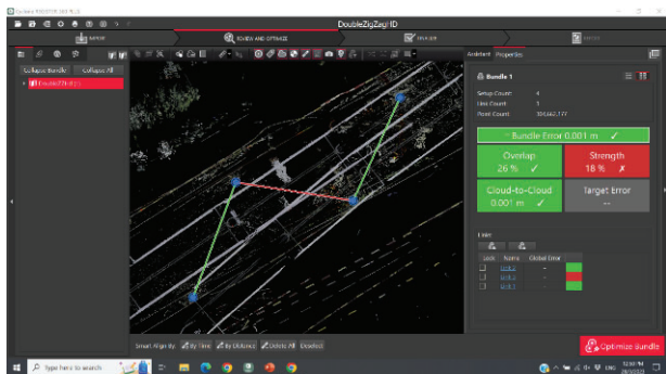
FIGURE 9. Output after importing raw data
