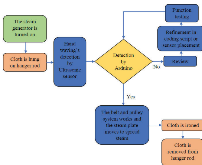
FIGURE 2. Function Structure Diagram
