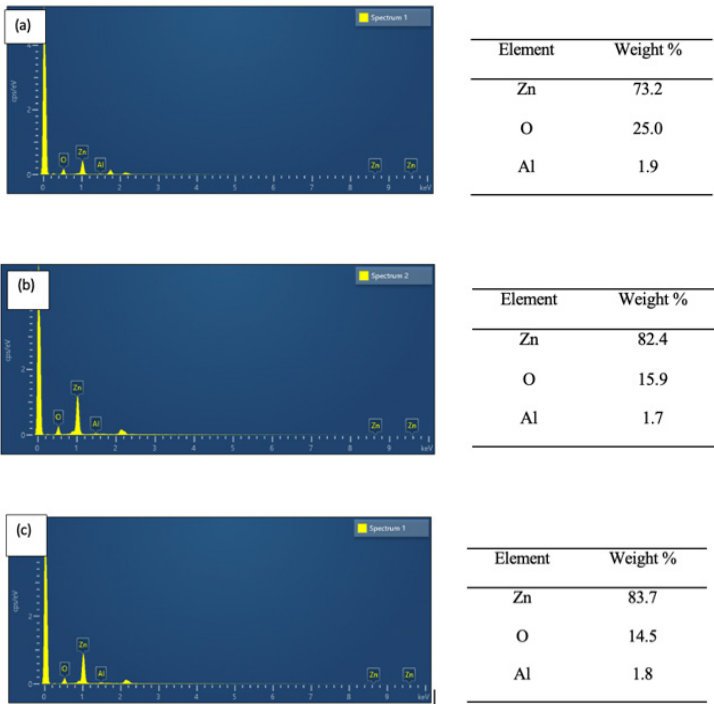
FIGURE 10. AZO thin film of EDS spectra and weight percentage on quartz at sputtering power of (a) 200 W, (b) 250 W and (c) 300 W
