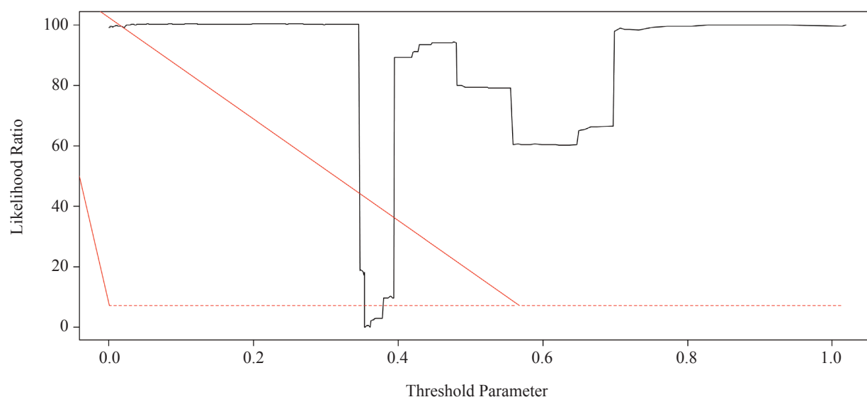
FIGURE 1. Confidence interval construction in single threshold model
