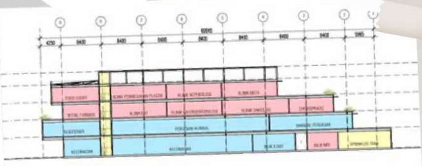
SECTION Y-Y
